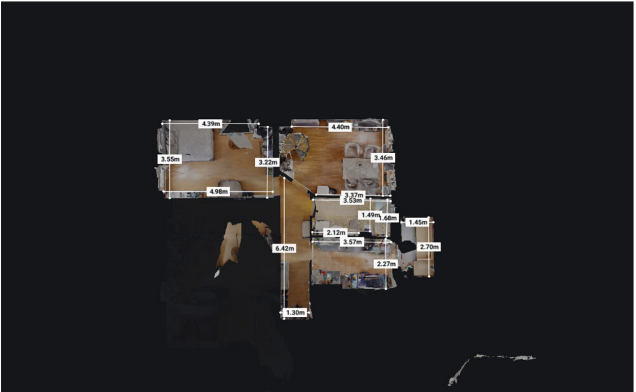
Grundriss_1
