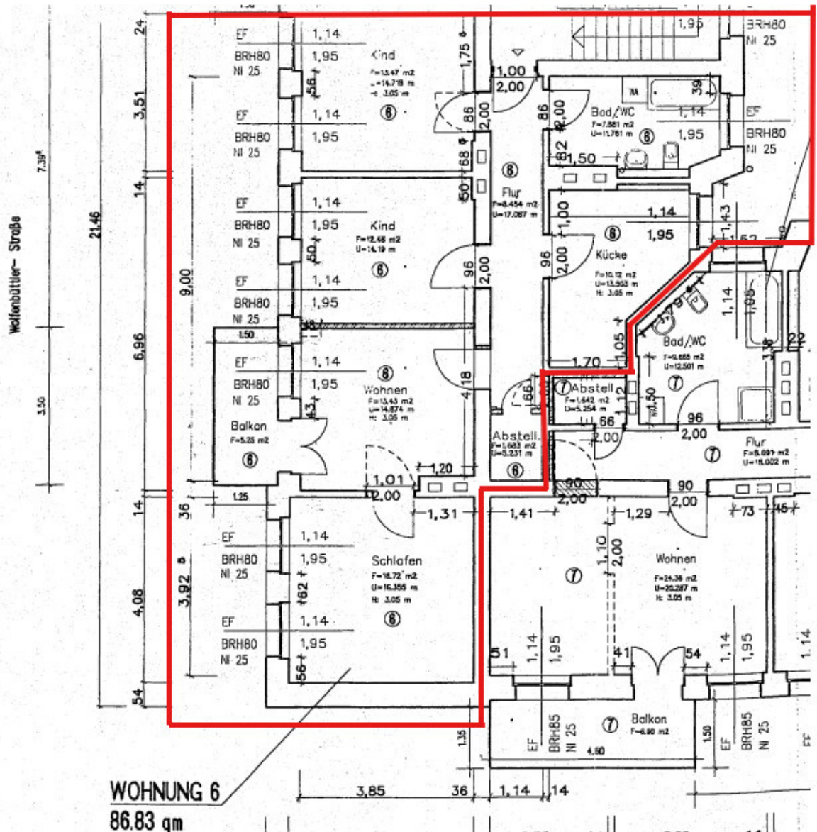
Grundriss_06
