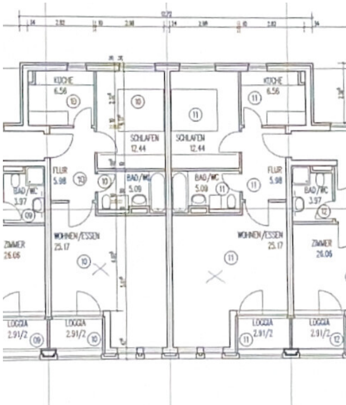
Grundrisse WE10+WE11
